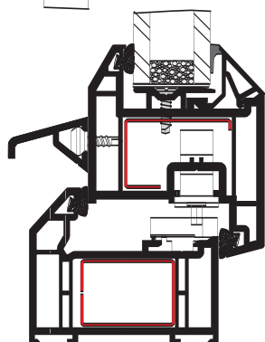
Cross Section through the Mock Sash
